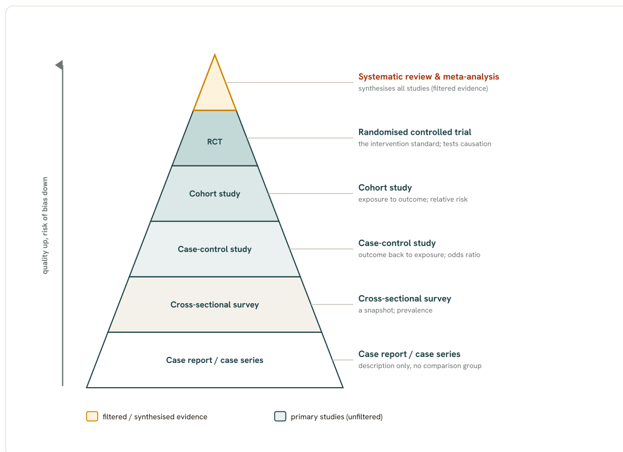
Fig 7.2 The hierarchy of evidence. Study designs rank by how well they control bias: the case report at the base offers only description, the observational designs add comparison groups, the randomised controlled trial adds the control of randomisation, and the systematic review with meta-analysis at the apex synthesises the whole body of filtered evidence. Reading a study begins with placing it on this pyramid, because the design sets the ceiling on the strength of the conclusion.
