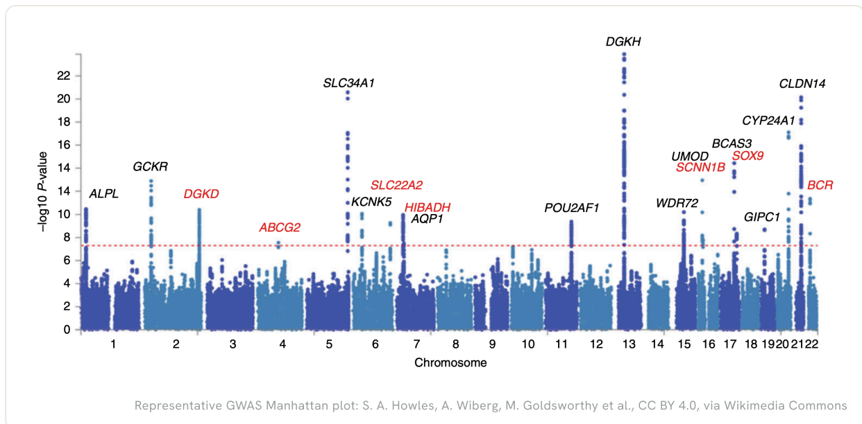
Fig 3.12 What a genome-wide association study produces: a Manhattan plot. Each dot is one single-nucleotide polymorphism, placed left to right by its position along the chromosomes, and its height is the strength of association (the negative log base ten of the p-value). The dashed horizontal line marks genome-wide significance ( 5 \times 10^{-8} ); the peaks rising above it are the associated loci. A psychiatric GWAS looks exactly like this: each significant peak adds only a sliver of risk, which a polygenic risk score later sums across the genome. The plot shown is a representative GWAS used to illustrate the method.
