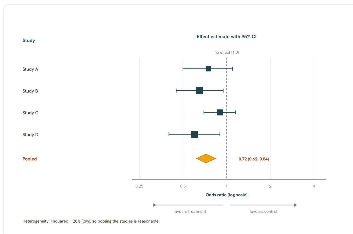
Fig 7.12 Reading a forest plot. Each study is a horizontal line (its 95% confidence interval) with a box marking the point estimate, the box sized by the study's weight in the pool. The vertical dashed line is the value of no effect. A confidence interval that crosses it is non-significant for that study. The diamond at the foot is the pooled estimate, its width the pooled confidence interval. Before trusting the pool, check heterogeneity: a high I-squared means the studies disagree and a single summary may mislead.
