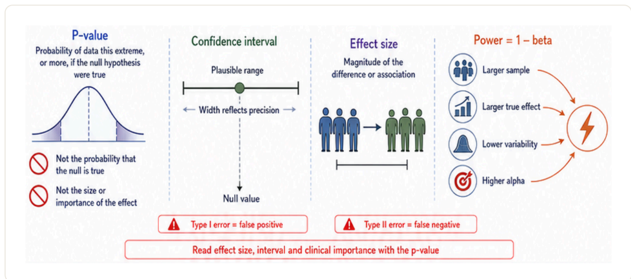
Fig 7.22 Inference: p-value, confidence interval, effect and power.
