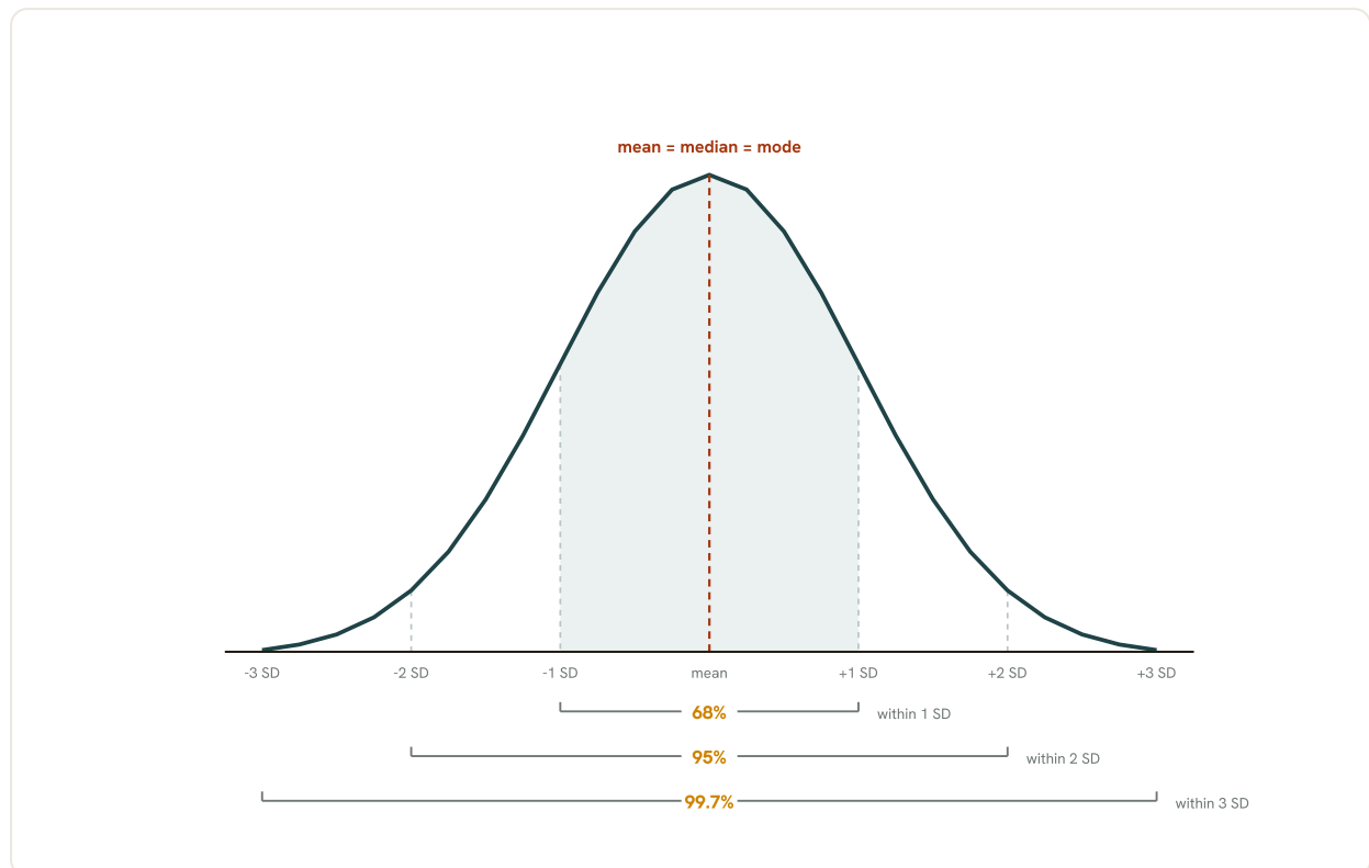
Fig 7.17 The normal curve and the empirical rule. In a normal distribution the mean, median and mode coincide at the peak and the spread is measured in standard deviations. The empirical rule fixes the proportions worth memorising: about 68 percent of observations lie within one SD of the mean, about 95 percent within two, and about 99.7 percent within three. The 95 percent band (more precisely 1.96 SD) is the basis of most confidence intervals and reference ranges.
