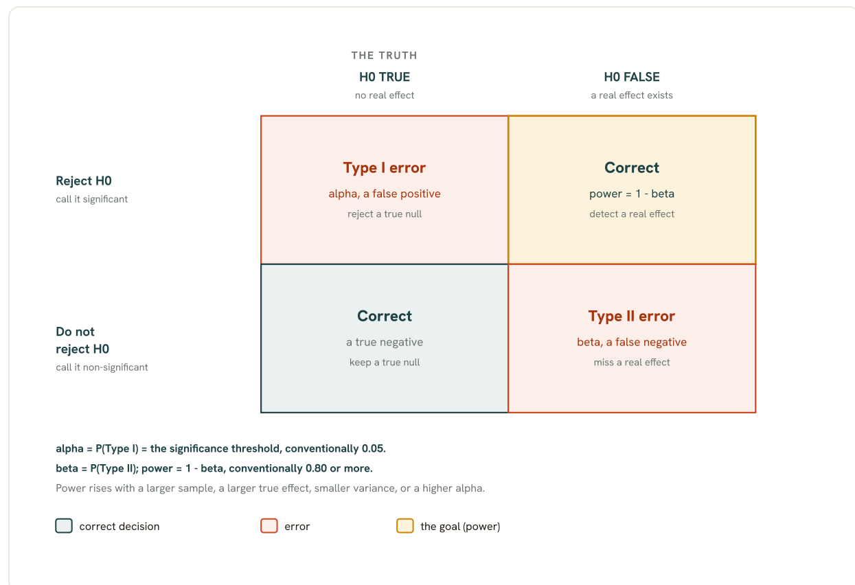
Fig 7.23 Type I and type II error. A test can go wrong two ways. Rejecting a null that is actually true is a type I error, a false positive, and its probability is alpha, the significance level we set. Failing to reject a null that is actually false is a type II error, a false negative, and its probability is beta. Power, the ability to detect a real effect, is one minus beta, and an underpowered study is the commonest reason a true effect is missed.
