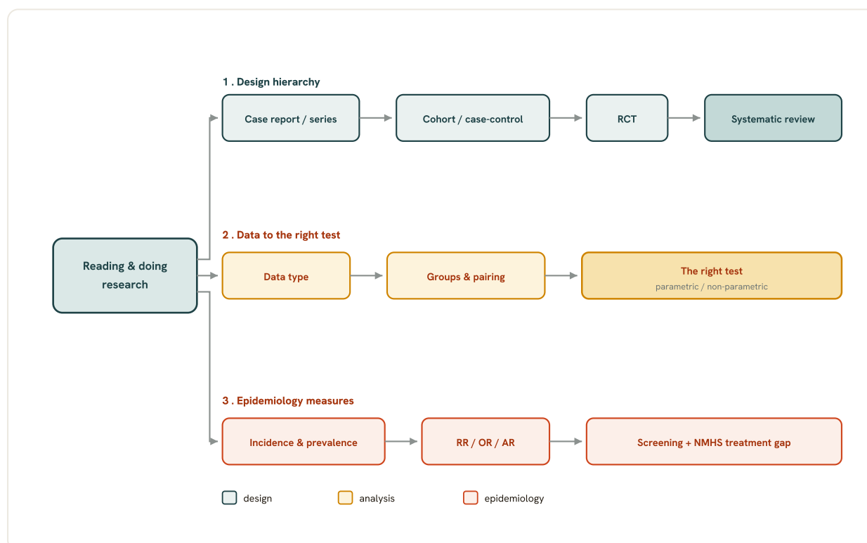
Fig 7.36 The whole-chapter synthesis map. Three branches run out from one hub: the design hierarchy that ranks the strength of a study, the analysis path that takes a dataset from its measurement scale through the number of groups to the correct test, and the epidemiology measures that quantify how common a disorder is and how strongly an exposure raises its risk. Cover the boxes and redraw the three branches from memory as the final retrieval check.
