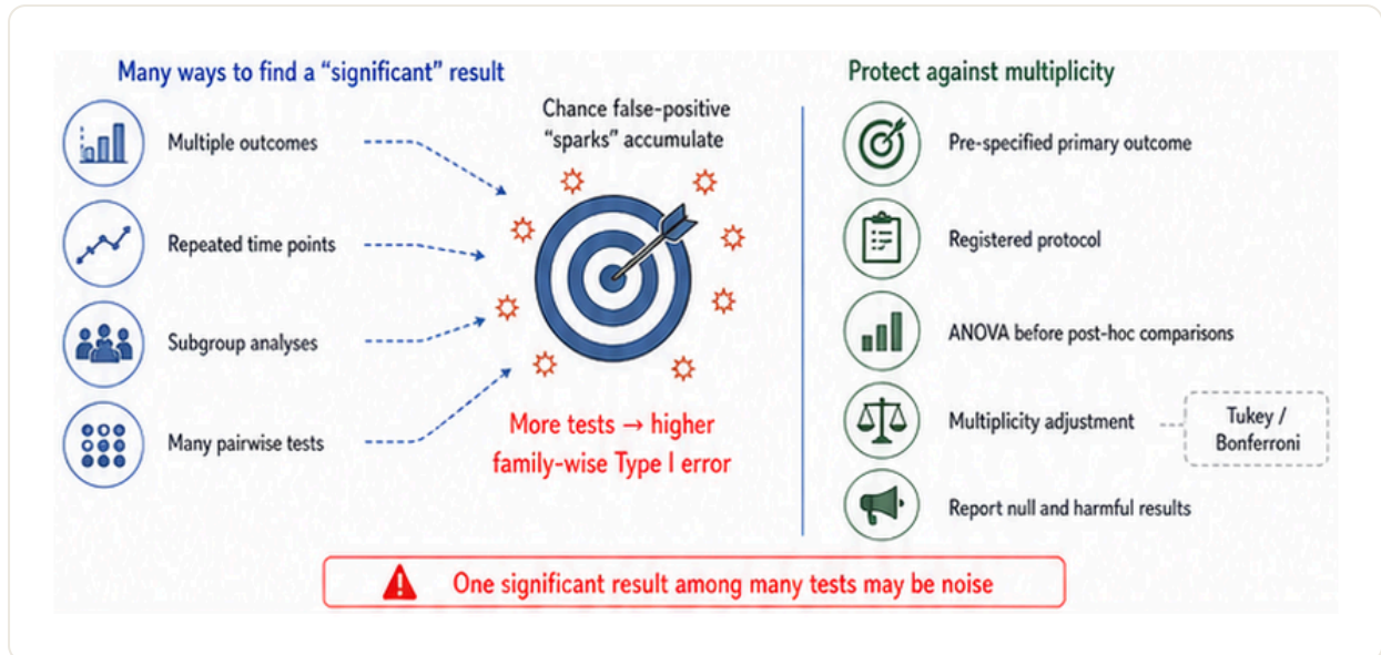
Fig 7.24 Multiplicity and selective reporting.
