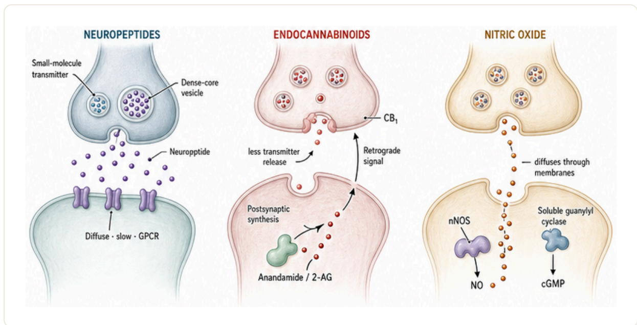
Fig 2.6 Unconventional neurotransmission.
